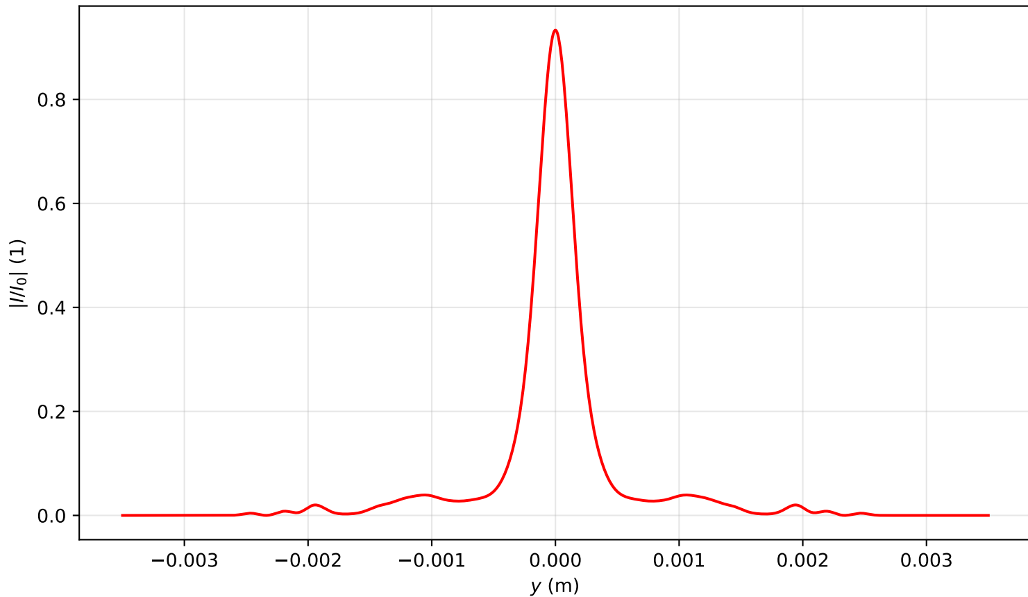
Intensity profile I(x=0, y, z=3.105)/I_0 , P_{in}=4.5P_{cr} , artificial time
